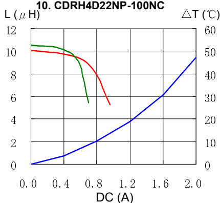
10. CDRH4D22NP-100NC
