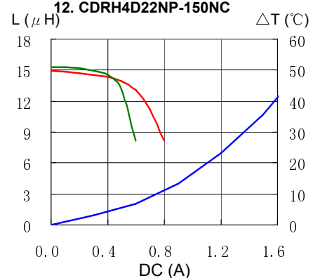
12. CDRH4D22NP-150NC
