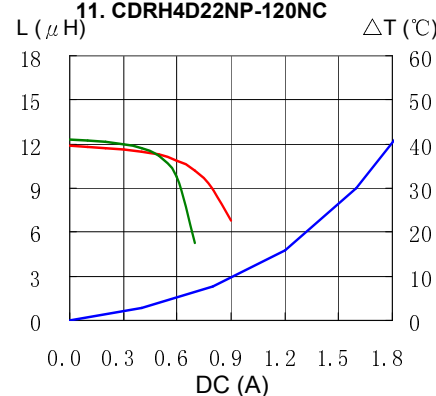
11. CDRH4D22NP-120NC
