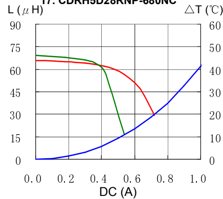
17. CDRH5D28RNP-680NC
